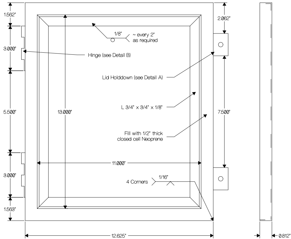
Lid Inside View
