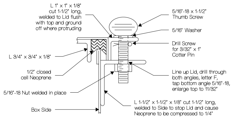
Detail A - Lid Holddown
