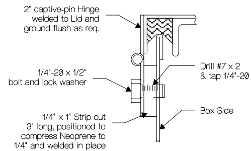
Detail B - Hinge Attachment
