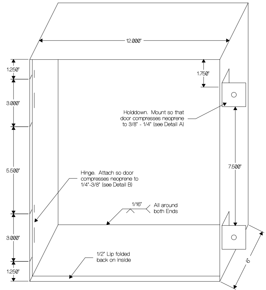
Box Construction
